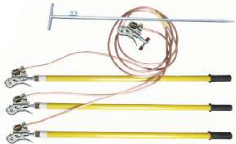
Grounding Set
